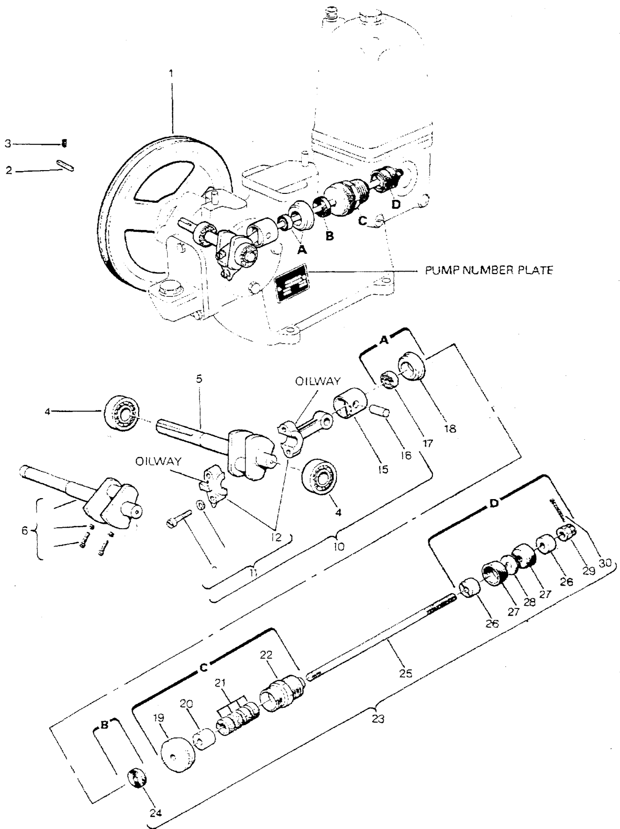
Fig.9 Connecting Rod and Plunger
